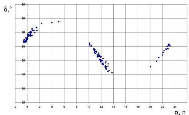
Figure 5: The position of abnormal radio 3C461 records varies depending on the distance between the Moon and the radio source by right ascension (1998-2004)
