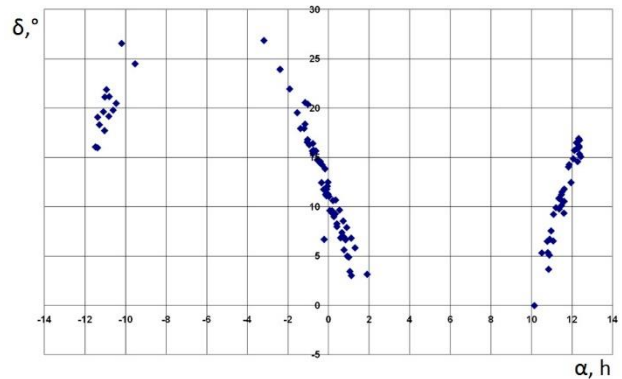
Figure 3: The position of abnormal radio 3C274 records varies depending on the distance between the Moon and the radio source by right ascension (1998-2004)
