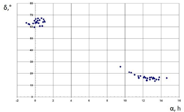
Figure 4: The position of abnormal radio 3C405 records varies depending on the distance between the Moon and the radio source by right ascension (1998-2004)
