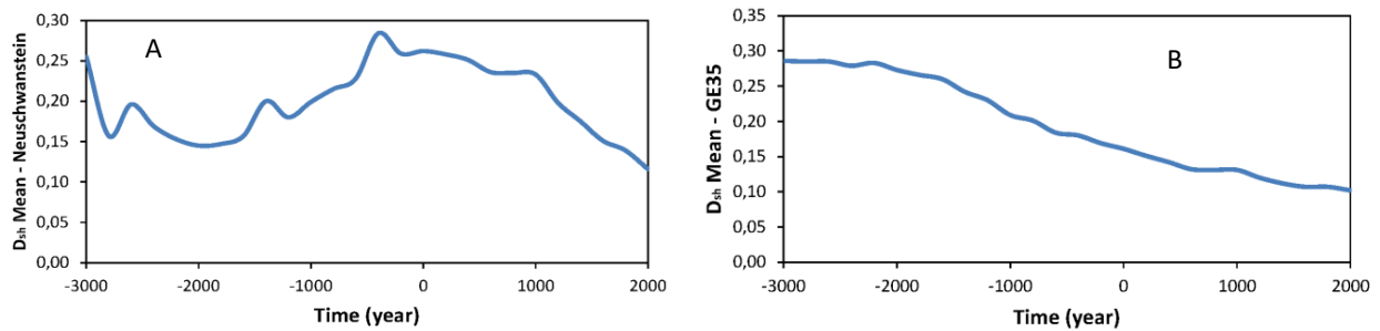
Figure 5: Evolution of the D_{SH} -criterion of similarity between the mean and Neuschwanstein meteorite orbits (A) and the mean and NEA 2010 GE35 orbits (B) over 5,000 years.
